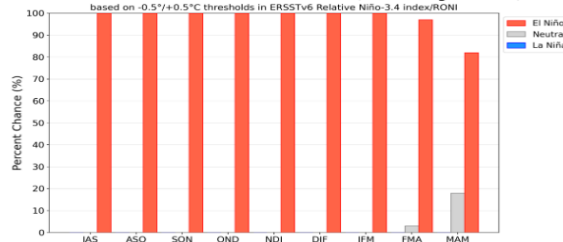
Official NOAA CPC ENSO Probabilities (issued August 2026)
