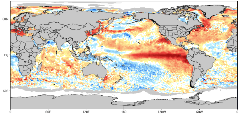
CDAS Sea Surface Temperature Anomaly (°C) (based on CFSR 1981-2010 Climatology) Analysis Time: 12z Sep 03 2026
