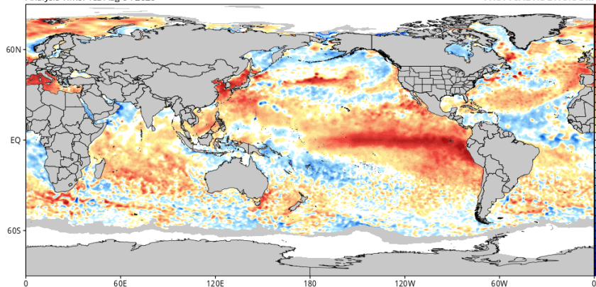
CDAS Sea Surface Temperature Anomaly (°C) (based on CFSR 1981-2010 Climatology) Analysis Time: 18z Aug 04 2026
