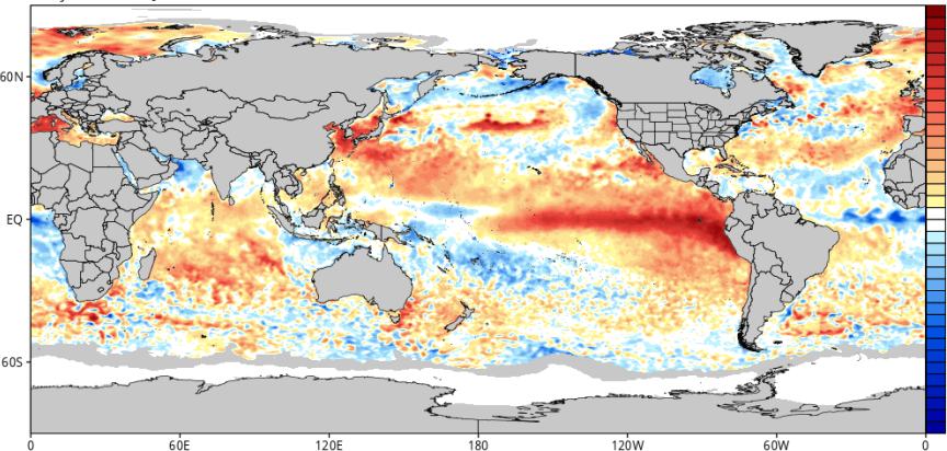
CDAS Sea Surface Temperature Anomaly (°C) (based on CFSR 1981-2010 Climatology) Analysis Time: 18z Jul 30 2026
