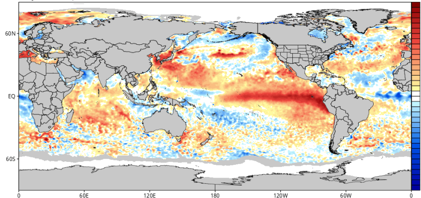
CDAS Sea Surface Temperature Anomaly (°C) (based on CFSR 1981-2010 Climatology) Analysis Time: 12z Jul 29 2026
