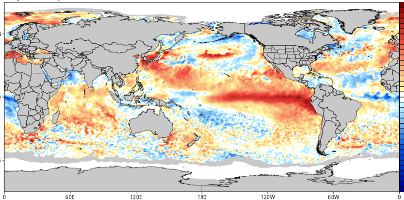
CDAS Sea Surface Temperature Anomaly (°C) (based on CFSR 1981-2010 Climatology) Analysis Time: 00z Jul 28 2026
