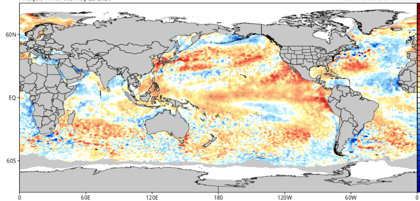
CDAS Sea Surface Temperature Anomaly (°C) (based on CFSR 1981-2010 Climatology) Analysis Time: 06z May 22, 2026
