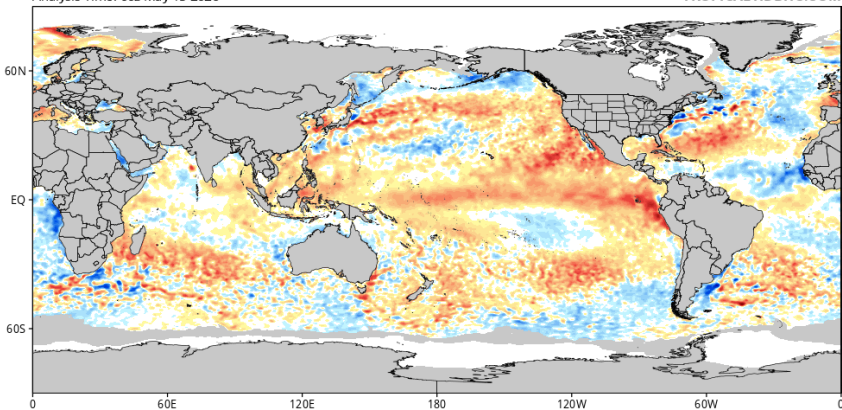
CDAS Sea Surface Temperature Anomaly (°C) (based on CFSR 1981-2010 Climatology) Analysis Time: 00z May 15 2026
