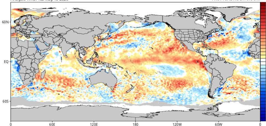
CDAS Sea Surface Temperature Anomaly (°C) (based on CFSR 1981-2010 Climatology) Analysis Time: 18z May 13 2026
