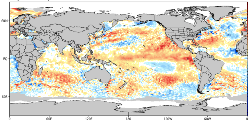
CDAS Sea Surface Temperature Anomaly (°C) (based on CFSR 1981-2010 Climatology) Analysis Time: 06z May 12 2026
