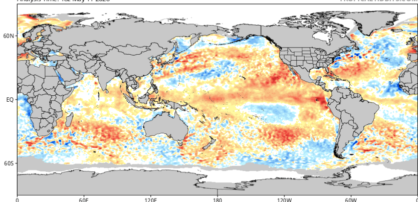
CDAS Sea Surface Temperature Anomaly (°C) (based on CFSR 1981-2010 Climatology) Analysis Time: 18z May 11 2026
