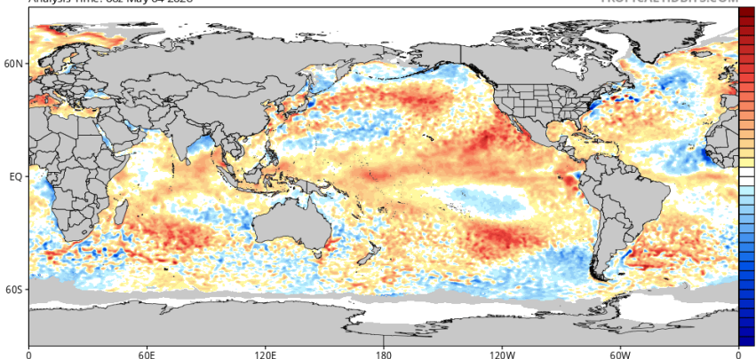
CDAS Sea Surface Temperature Anomaly (°C) (based on CFSR 1981-2010 Climatology) Analysis Time: 06z May 04 2026
