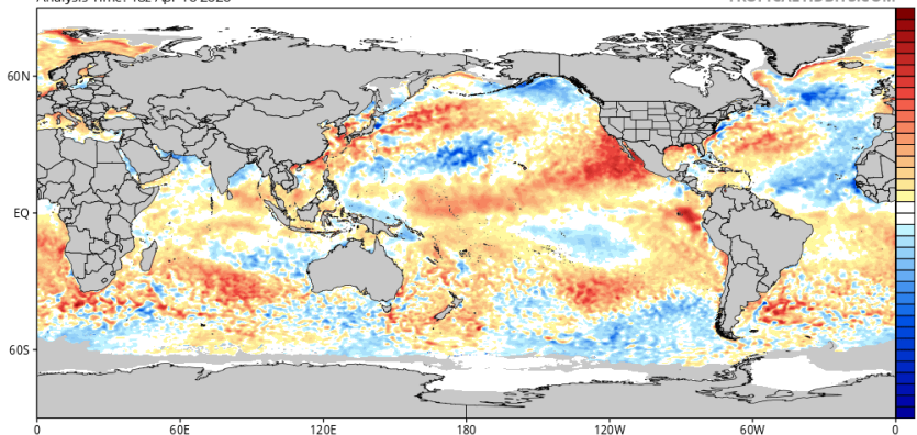
CDAS Sea Surface Temperature Anomaly (°C) (based on CFSR 1981-2010 Climatology) Analysis Time: 18z Apr 16 2026
