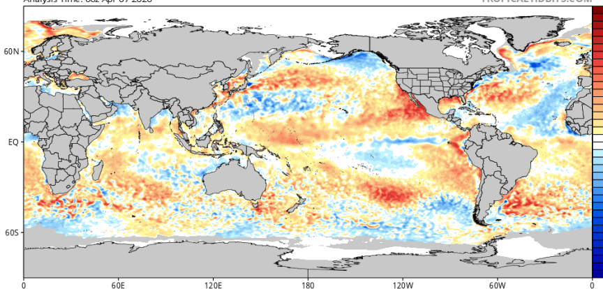
CDAS Sea Surface Temperature Anomaly (°C) (based on CFSR 1981-2010 Climatology) Analysis Time: 06z Apr 07 2026
