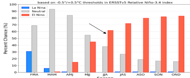
Official NOAA CPC ENSO Probabilities (issued March 2026) based on -0.5/+0.5°C thresholds in ERSSTv5 Relative Niño-3.4 index
