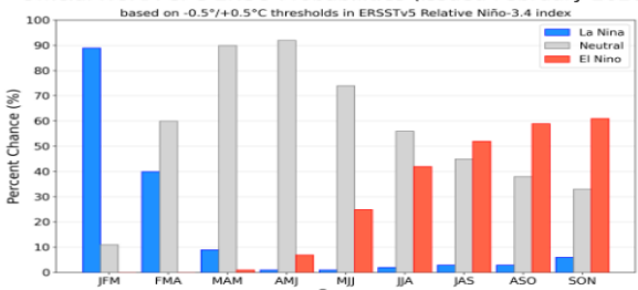
Official NOAA CPC ENSO Probabilities (issued February 2026)
