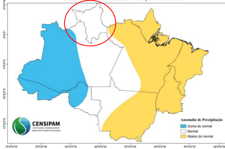
Figura 2 ( https://panorama.sipam.gov.br/panorama/pages/boletimClima.html )
