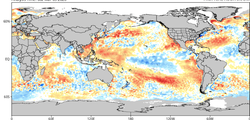
CDAS Sea Surface Temperature Anomaly (°C) (based on CFSR 1981-2010 Climatology) Analysis Time: 06z Mar 05 2026
