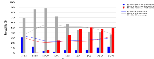
Mid-January 2026 IRI Model-Based Probabilistic ENSO Forecasts
