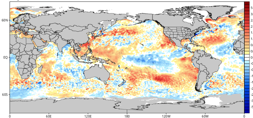
CDAS Sea Surface Temperature Anomaly (°C) (based on CFSR 1981-2010 Climatology) Analysis Time: 06z Mar 03 2026
