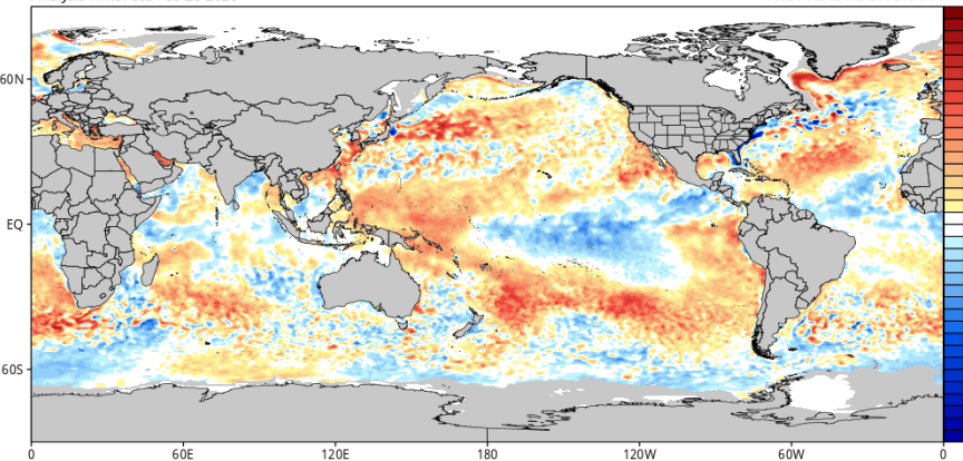
CDAS Sea Surface Temperature Anomaly (°C) (based on CFSR 1981-2010 Climatology) Analysis Time: 00z Feb 26 2026
