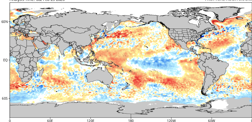
CDAS Sea Surface Temperature Anomaly (°C) (based on CFSR 1981-2010 Climatology) Analysis Time: 06z Feb 25 2026
