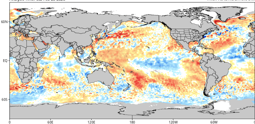
CDAS Sea Surface Temperature Anomaly (°C) (based on CFSR 1981-2010 Climatology) Analysis Time: 06z Feb 23 2026
