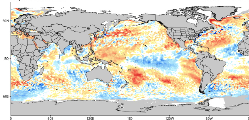
CDAS Sea Surface Temperature Anomaly (°C) (based on CFSR 1981-2010 Climatology) Analysis Time: 06z Feb 19 2026
