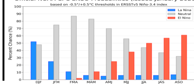
Official NOAA CPC ENSO Probabilities (issued January 2026)
