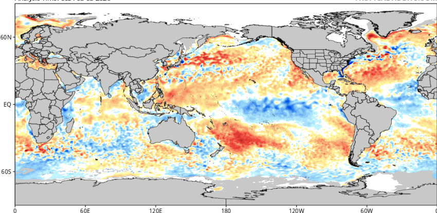
CDAS Sea Surface Temperature Anomaly (°C) (based on CFSR 1981-2010 Climatology) Analysis Time: 00z Feb 03 2026
