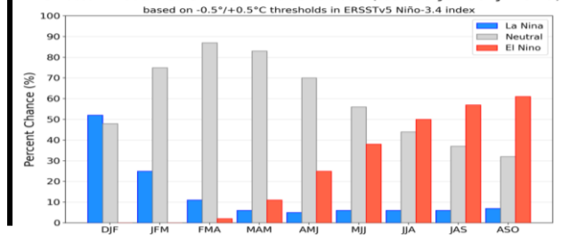
Official NOAA CPC ENSO Probabilities (issued January 2026)
