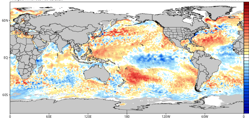
CDAS Sea Surface Temperature Anomaly (°C) (based on CFSR 1981-2010 Climatology) Analysis Time: 00z Feb 02 2026
