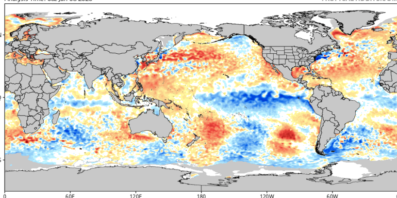
CDAS Sea Surface Temperature Anomaly (°C) (based on CFSR 1981-2010 Climatology) Analysis Time: 06z Jan 08 2026
