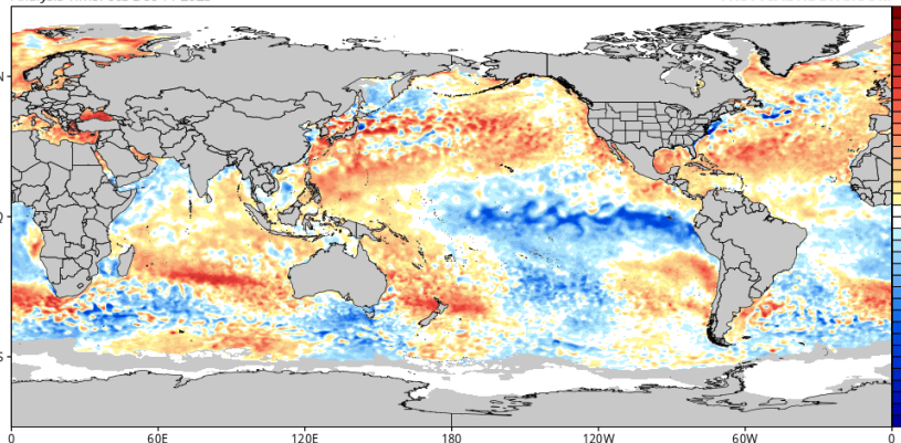
CDAS Sea Surface Temperature Anomaly (°C) (based on CFSR 1981-2010 Climatology) Analysis Time: 06z Dec 11 2025
