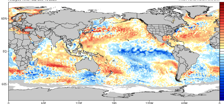
CDAS Sea Surface Temperature Anomaly (°C) (based on CFSR 1981-2010 Climatology) Analysis Time: 06z Dec 10 2025
