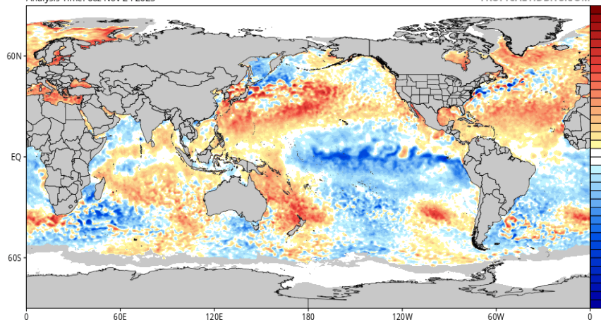
CDAS Sea Surface Temperature Anomaly (°C) (based on CFSR 1981-2010 Climatology) Analysis Time: 06z Nov 24 2025
