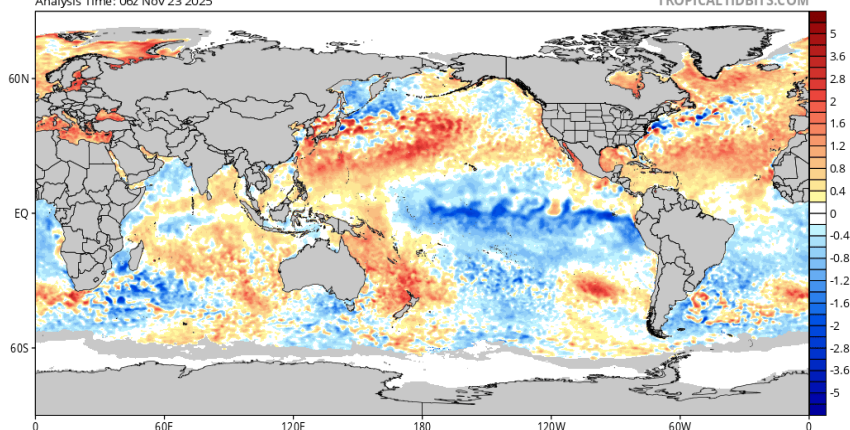
CDAS Sea Surface Temperature Anomaly (°C) (based on CFSR 1981-2010 Climatology) Analysis Time: 06z Nov 23 2025
