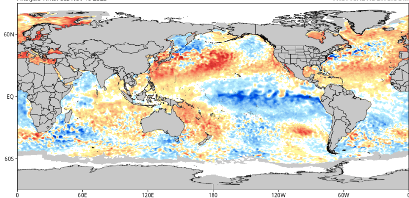
CDAS Sea Surface Temperature Anomaly (°C) (based on CFSR 1981-2010 Climatology) Analysis Time: 06z Nov 19 2025
