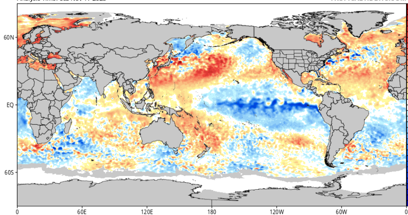
CDAS Sea Surface Temperature Anomaly (°C) (based on CFSR 1981-2010 Climatology) Analysis Time: 06z Nov 17 2025
