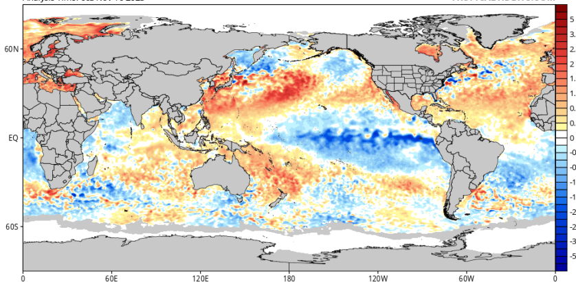
CDAS Sea Surface Temperature Anomaly (°C) (based on CFSR 1981-2010 Climatology) Analysis Time: 06z Nov 16 2025
