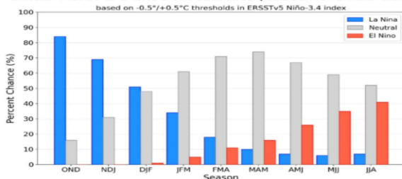
Official NOAA CPC ENSO Probabilities (issued November 2025)
