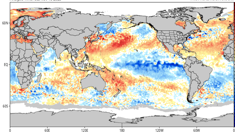
CDAS Sea Surface Temperature Anomaly (°C) (based on CFSR 1981-2010 Climatology) Analysis Time: 00z Nov 15 2025
