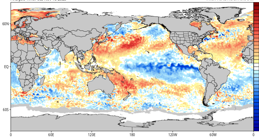
CDAS Sea Surface Temperature Anomaly (°C) (based on CFSR 1981-2010 Climatology) Analysis Time: 06z Nov 13 2025
