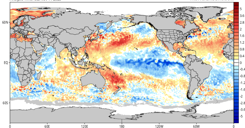
CDAS Sea Surface Temperature Anomaly (°C) (based on CFSR 1981-2010 Climatology)
