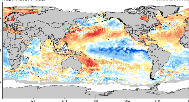
CDAS Sea Surface Temperature Anomaly (°C) (based on CFSR 1981-2010 Climatology) Analysis Time: 06z Nov 10 2025
