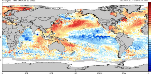
CDAS Sea Surface Temperature Anomaly (°C) (based on CFSR 1981-2010 Climatology)
