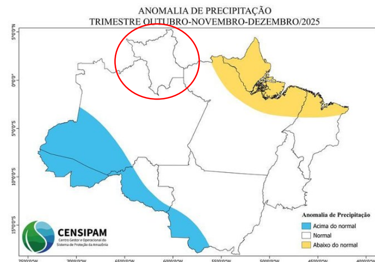
Figura 2 ( https://panorama.sipam.gov.br/panorama/pages/boletimClima.html )
