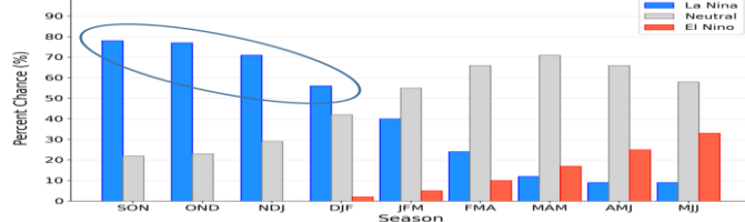
Official NOAA CPC ENSO Probabilities (issued October 2025) based on -0.5/+0.5°C thresholds in ERSSTv5 Niño-3.4 index
