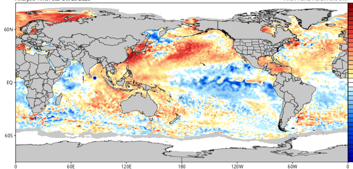
CDAS Sea Surface Temperature Anomaly (°C) (based on CFSR 1981-2010 Climatology) Analysis Time: 06z Oct 20 2025
