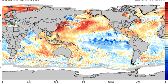
CDAS Sea Surface Temperature Anomaly (°C) (based on CFSR 1981-2010 Climatology) Analysis Time: 06z Oct 17 2025
